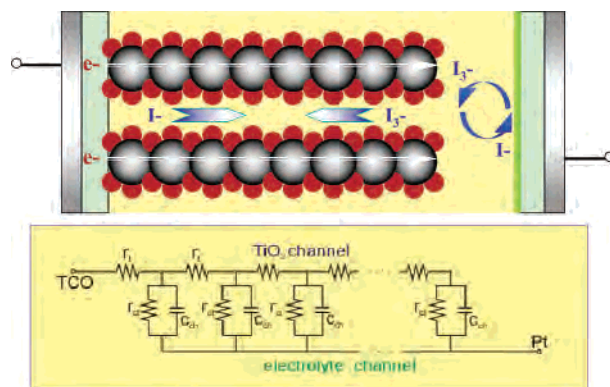
Figure 4. Transmission line description of the conduction band electron motion through a network of mesoscopic semiconductor particles.
