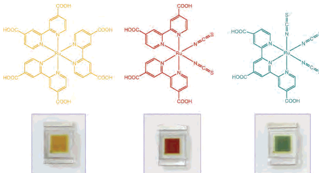
Figure 5. Structure of the ruthenium sensitizers \text{RuL}_3 (yellow) cis - \text{RuL}_2(\text{NCS})_2 (red) and \text{RuL}'(\text{NCS})_3 (green) where \text{L} = 2,2' -bipyridyl-4,4'-dicarboxylic acid and \text{L}' = 2,2',2'' -terpyridyl-4,4',4''-tricarboxylic acid. The lower part of the picture shows nanocrystalline \text{TiO}_2 films loaded with a monolayer of the respective sensitizer. The film thickness is 5 \mu\text{m} .
