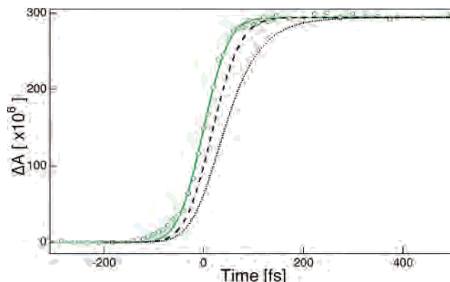
Figure 7. Transient absorption signal for N-719 adsorbed on nanocrystalline titania (○) (pump wavelength 535 nm; probe 860 nm). The fitted instrument response is 57 fs (—). The simulated exponential rises with time constants of 20 fs (---) and 50 fs (···) and convoluted with the same instrument response are shown.
