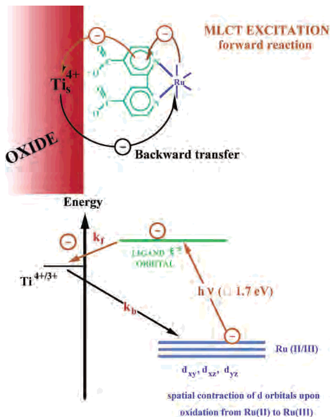
Figure 6. Interfacial electron transfer involving a ruthenium complex bound to the surface of TiO 2 via a carboxylated bipyridyl ligand. Orbital diagram for the forward electron injection (rate constant k_f ) from the \pi^* orbital of the bipyridyl ligand into the empty t_{2g} orbitals forming the TiO 2 conduction band and the backward electron transfer from the conduction band of the oxide into the Ru(III) d orbitals.
